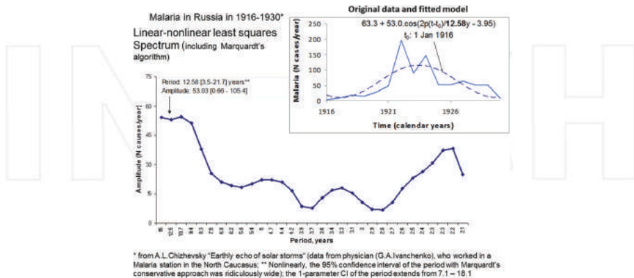
Figure 7. A decadal component characterizes the incidence of malaria in Russia between 1916 and 1930, as seen from the low-frequency spectral peak, resolved nonlinearly as an about 12.6-year component, which is fitted to the data (top right). Note a secondary smaller spectral peak corresponding to a period of about 2.3 years, as observed also in the data from Burundi ( Figure 1 ) and Papua New Guinea ( Figure 3 ). © Halberg Chronobiology Center.
