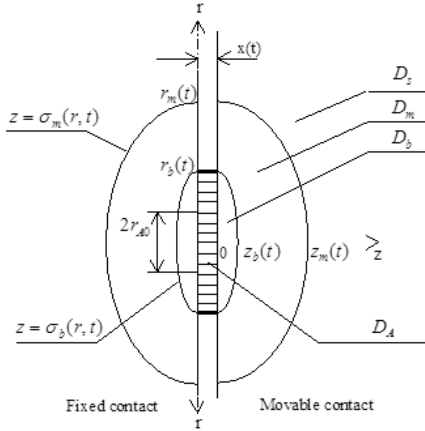
Fig.1 The arc and contacts geometry: arc region D_A , evaporated zone D_b , solid zone D_s
