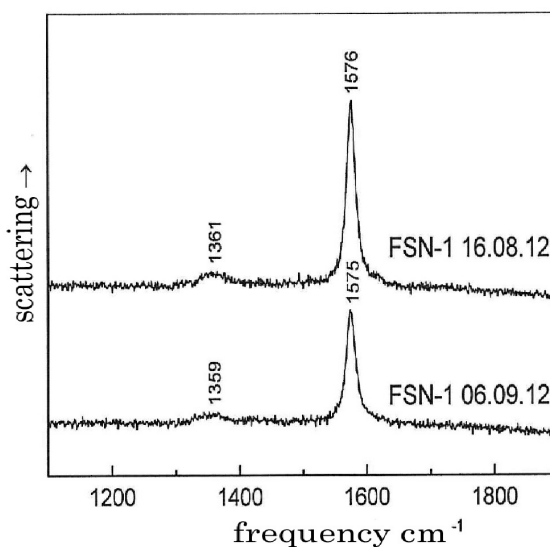
Figure 3. Raman spectra of anode powders
