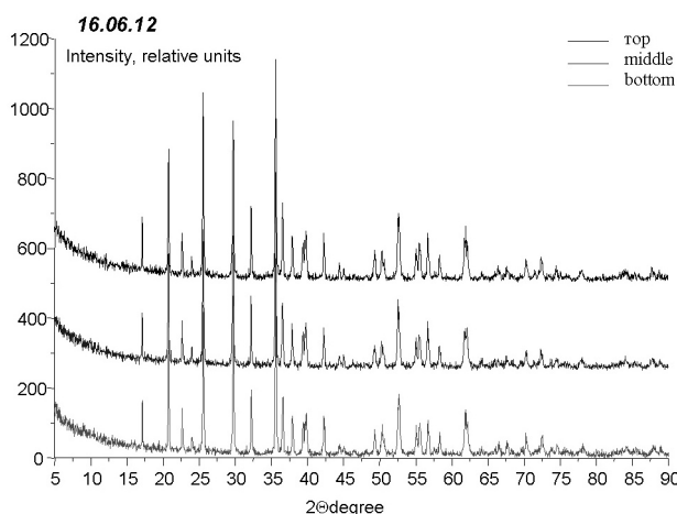
Figure 1. XRD pattern of \text{LiFePO}_4 cathode powder
