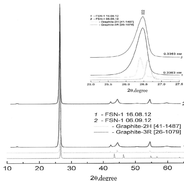
Figure 2. Anode powder diffractograms
