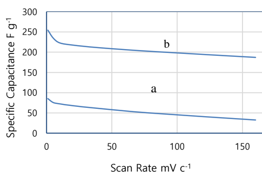
Figure 1. The specific capacitance of physical (a) and chemical (b) activated CRH based electrodes calculated from CV
