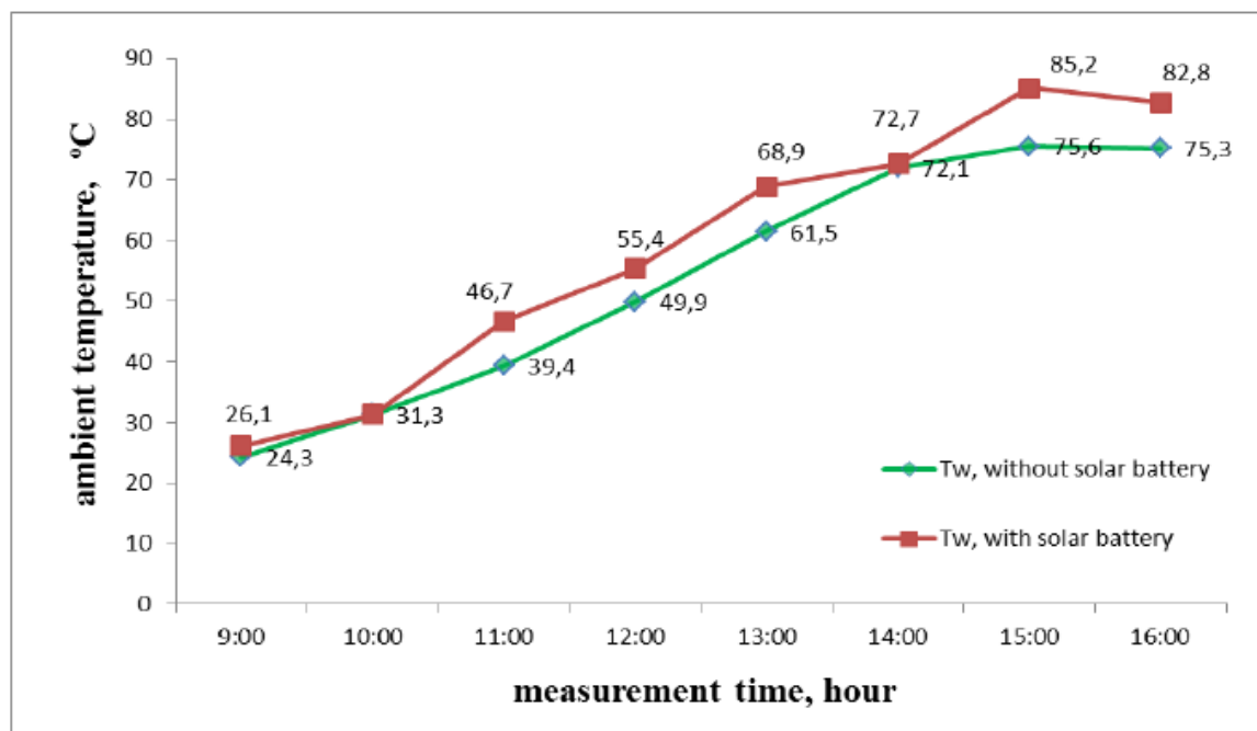
Figure 4. Change in temperature of oily waste using solar energy
