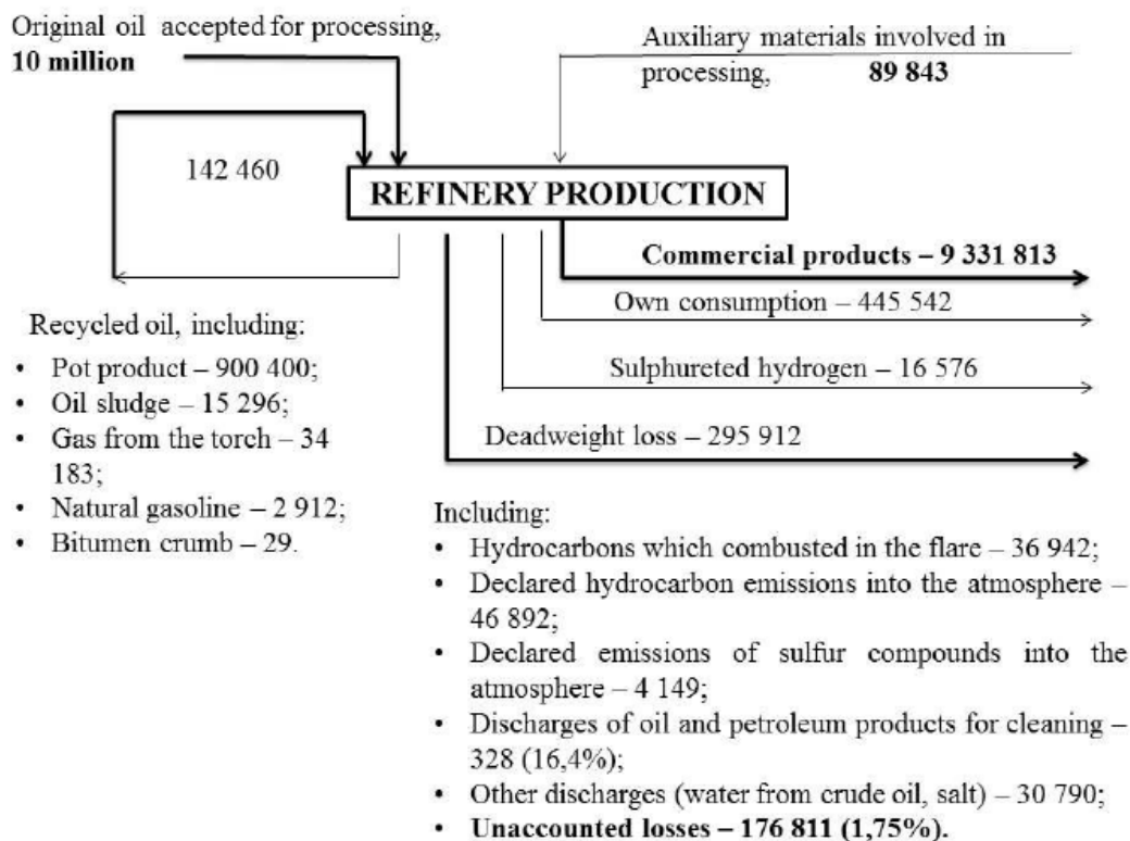
Figure 1. General scheme of input and output material courses refinery (tons/year)
