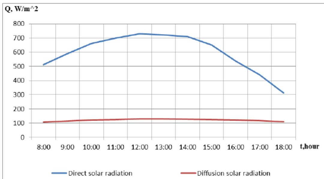
Figure 3. Graphs of direct and diffuse solar radiation during the light of a sunny day in July, the month
