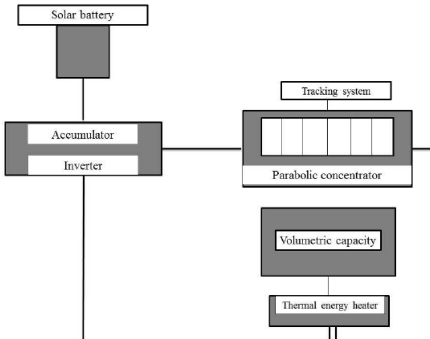
Figure 2. Schematic diagram of solar device equipped with concentrating elements
