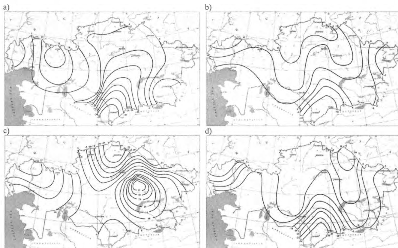
Fig. 5. Composition fields of precipitation abnormalities in the middle months of the seasons in the years of El Nino (a – spring; c – summer) and following the year of El Nino (b – spring; d – summer)
