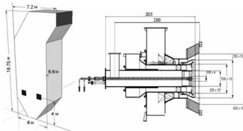
Fig. 2. The general form of the combustion chamber and coal-dust burner
