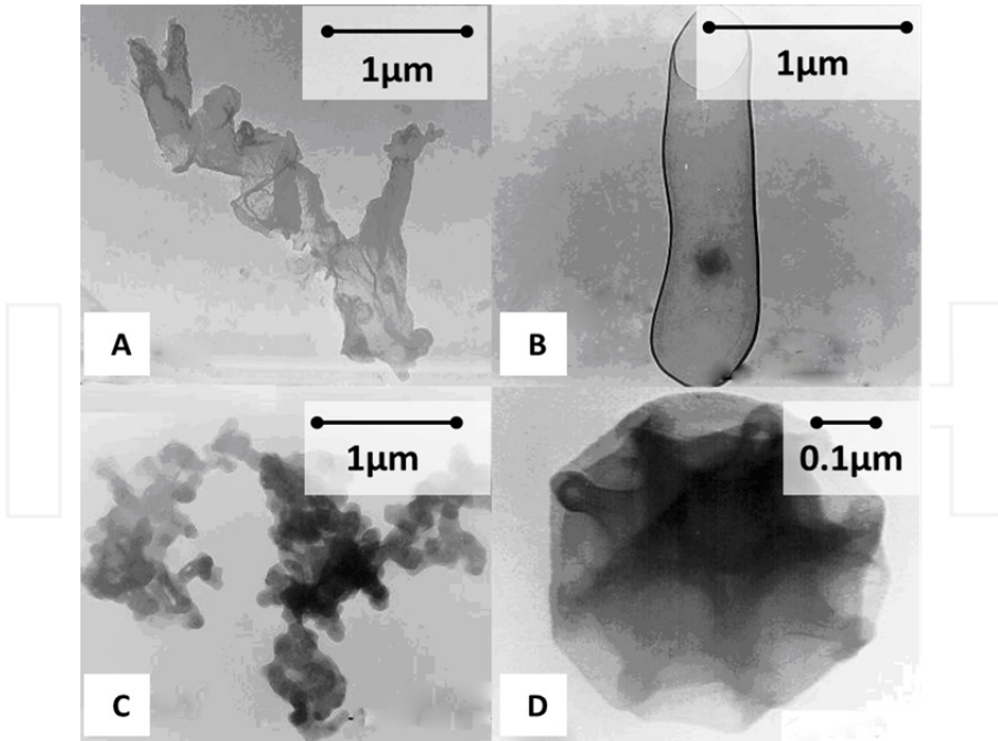
Figure 3. Diverse micro- and nanoscale structures observed with electron microscopy in apricot stones carbonized at different temperatures: (A) at 500°C; (B) at 600°C for 30 min; (C) at 700°C; (D) at 750°C.
