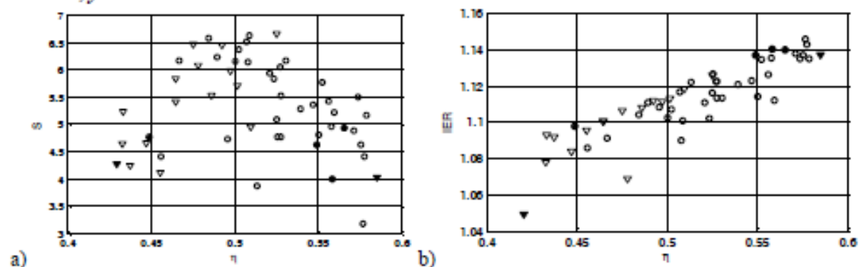
Figure 2. Dependence of information entropy (a) and information-to-entropy ratio (b) on porosity of SiNW films: \circ – "white" silicon (top view); \nabla – "white" silicon (lateral view); \bullet – "black" silicon (top view); \blacktriangledown – "black" silicon (lateral view).
