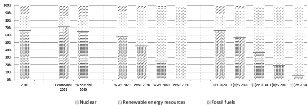
Fig. 2.5: Share of primary energy sources in world electricity generation, %
