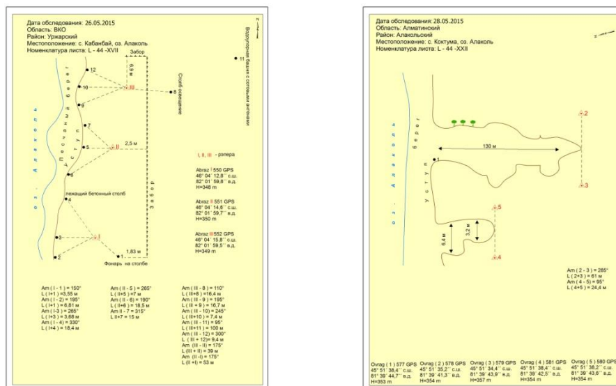
Figure 6. Setting the vielbein by the profile. (a) Kabanbai village, b) Koktuma village)
