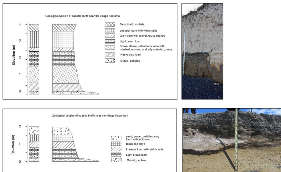
Figure 2. Geological section of costal bluffs near the village Koktuma and Kabanbay
