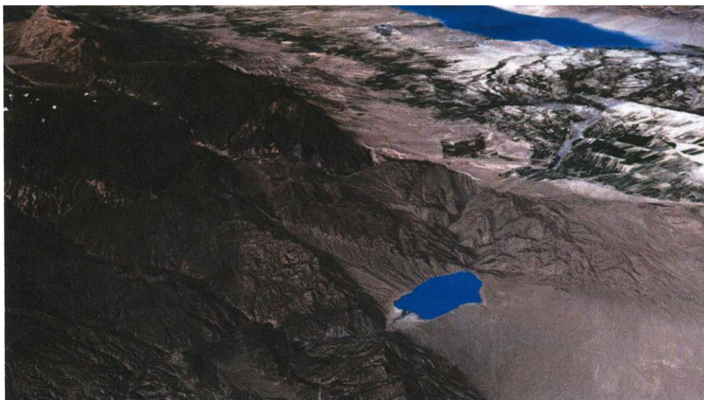
Figure 6. Bartogay water tank (Terrain Model from Google Planet Earth 7.1.1.1988)
