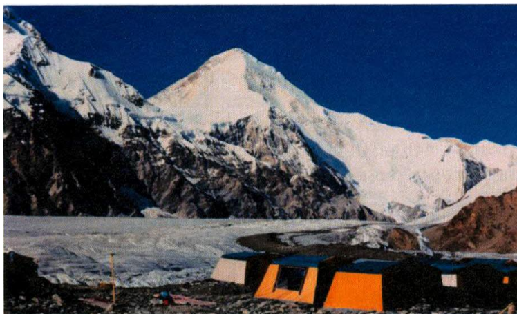
Figure 4. Nival-glacial exomorphogenesis zone of Tien Shan, Khan-Tengri peak (photo by Veselova L. K.)
