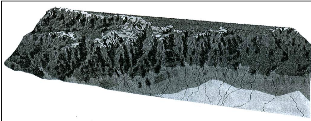
Figure 2. 3D-model of Ile Alatau climate zonation in ArcScene
