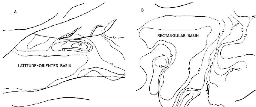
Figure 5. Physiographic types of intermontane basins of the Northern Tien Shan
