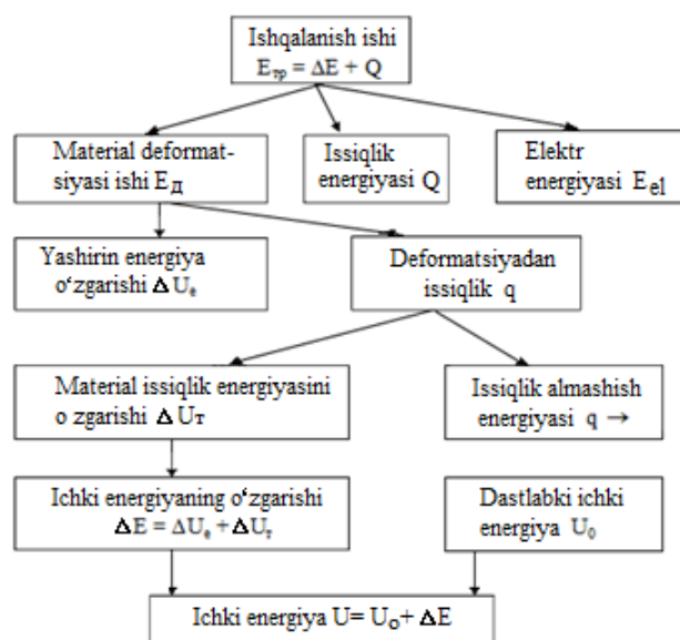
2- rasm. Ishqalanish va yeyilish jaryonining energiya balansi sxemasi
