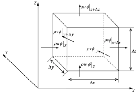
Fig. 4. Control volume for the generalized transport equation.
