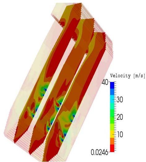
Fig. 10. Velocity profile on the different levels of the combustion chamber Y_1 = 2.85 m, Y_2 = 7.2 m, Y_3 = 11.69 m on the Y axis for two layers ( z_1 = 6.2 m) and ( z_2 = 10.75 m).
