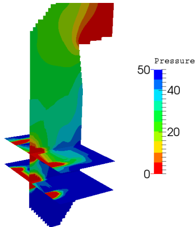
Fig. 12. Pressure profile by the height of combustion chamber.
