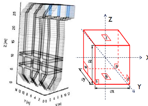
Fig. 3. The scheme of the boiler separated with control volume and elementary control cell.
