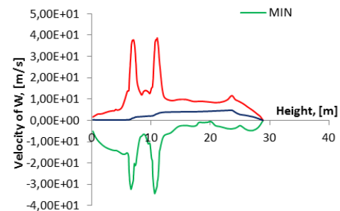
Fig. 7. Distribution of the vector velocity direction of the Z axis height of the combustion chamber of the boiler BKZ-420.
