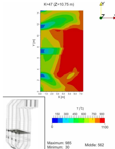
Fig. 14. Temperature distribution in the cross section ( z = 10.75 m) of the upper tier of the combustion chamber of the boiler BKZ-420.
