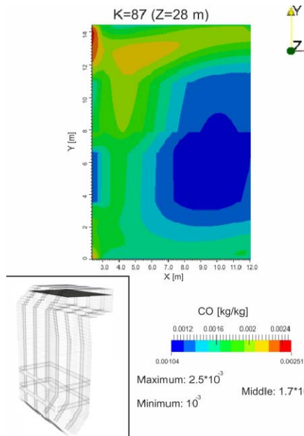
Fig. 16. Distribution of CO concentration at the outlet ( z = 28 m) from the furnace combustion boiler BKZ-420.
