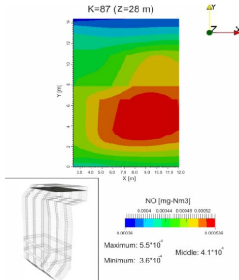
Fig. 20. Distribution of NO concentration at the outlet ( z = 28 m) from the furnace combustion boiler BKZ-420.
