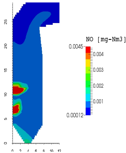
Fig. 19. Distribution of the concentration of NO in the longitudinal section ( y = 7.21 m) of the combustion chamber of the boiler BKZ-420.
