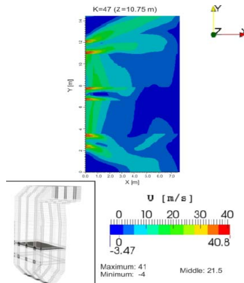
Fig. 8. Velocity profile on the cross section of the combustion chamber of the boiler BKZ-420 (K=47, Z = 10.75m).
