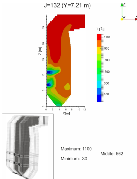
Fig. 13. Temperature distribution in the longitudinal section ( y = 7.21 m) of the combustion chamber of the boiler BKZ-420,
