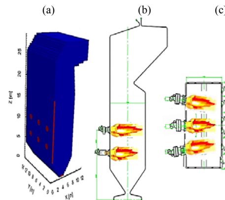
Fig. 2. General view of the industrial boiler BKZ-420 of the Almaty TPP-2. (a)3D view of BKZ-420 boiler and its breakdown into control volumes; (b) burners establish arranged on two levels; (c) top view on the cross section (h = 10.75m).
