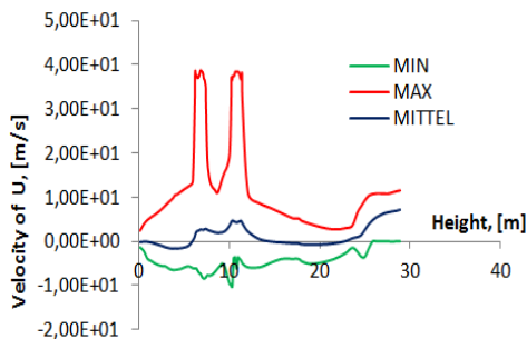
Fig. 5. Distribution of the velocity vector direction of the x axis height of the combustion chamber of the boiler BKZ-420-140-7C.
