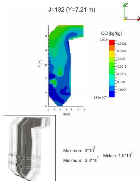
Fig. 15. Distribution of the concentration of CO in the longitudinal section ( y = 7.21 m) of the combustion chamber of the boiler BKZ-420.
