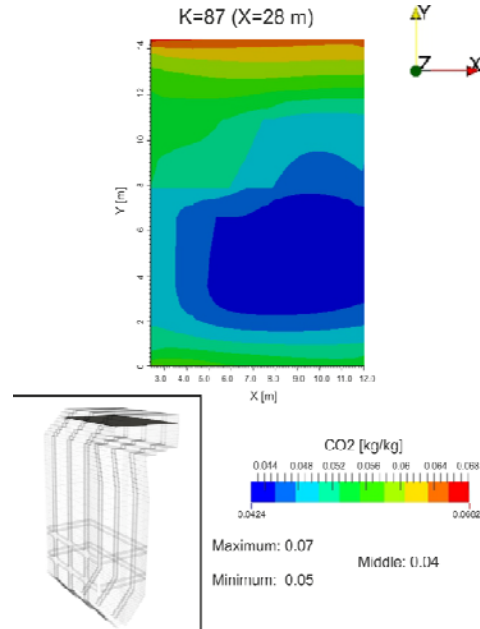
Fig. 18. Distribution of \text{CO}_2 concentration at the outlet ( z = 28 m) from the furnace combustion boiler BKZ-420.
