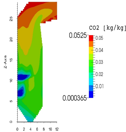
Fig. 17. Distribution of the concentration of \text{CO}_2 in the longitudinal section ( y = 7.21 m) of the combustion chamber of the boiler BKZ-420.
