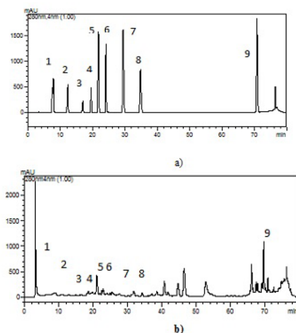
Figure 1 – HPLC profiles: a) chromatogram of the standards; b) chromatogram of the phenolic compounds in ethanol extract from the aerial part of C. alatavicus :
