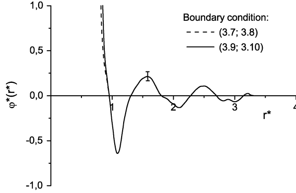
Figure 6. Effective interaction potential for dusty particles. Experiment No. 1.
