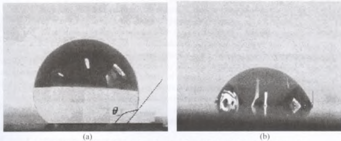
Fig. 3. (a) A drop of liquid placed on the central superhydrophobic region (zone 1) of the surface shown in Fig. 2, and (b) a more hydrophilic bare Si wafer surface.
