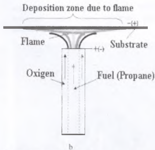
Fig. 1. Image and schematic representation of the burning experimental setup.
