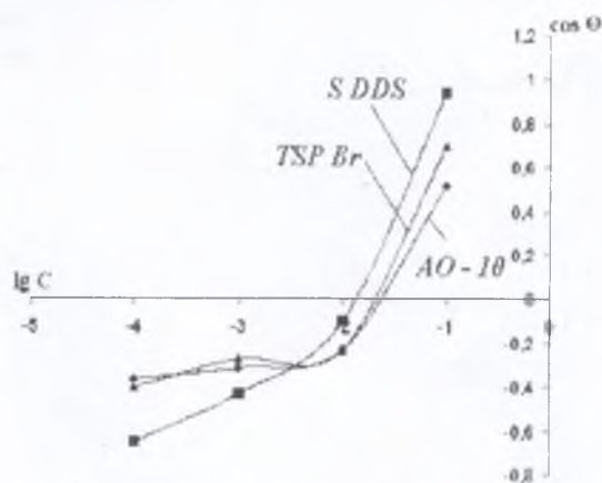
Fig. 6. Variation of the contact angle versus the logarithm of concentration
