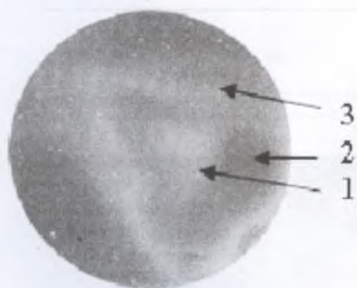
Fig. 2. A Si disc with carbon nanobead coating after 4 min exposure to the flame showing three deposition zones (1, 2 and 3).
