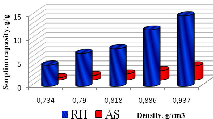
Figure 3. Dependence between adsorbate density and sorption capacity for carbonized rice husks (RH) and apricot stone (AS) carbonized at 700 °C
