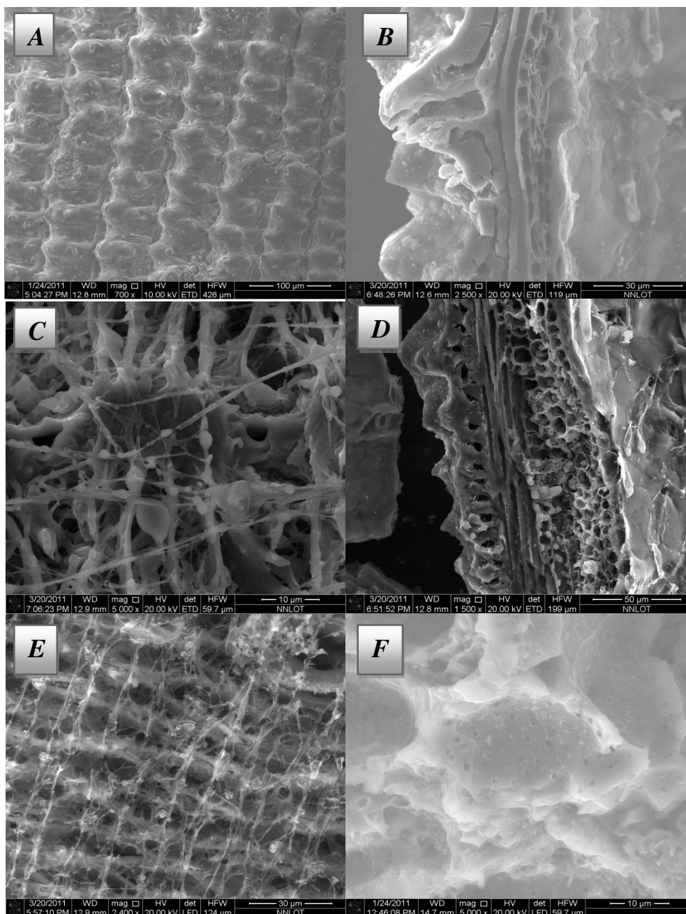
Figure 2. SEM images of CRH and CAS; CRH at 400°C (A, B, C), CRH at 700°C (D, E) and CAS at 700 °C (F)
