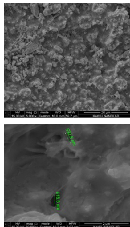
Fig. 5. SEM-images of the combustion products of the BaCrO 4 /TiB 2 system
