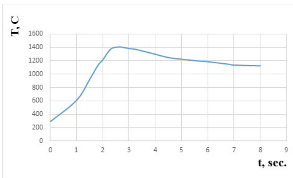
Fig. 4. Influence of the burning time of a slowly burning mixture of the BaCrO 4 /TiB 2 system on the temperature.
