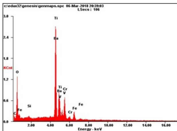
Fig. 7. EDX analysis of products of the \text{BaCrO}_4/\text{TiB}_2 system combustion.
