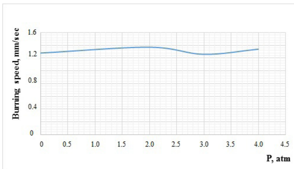
Fig. 3. Effect of pressure on the combustion rate of the \text{BaCrO}_4/\text{TiB}_2 system.
