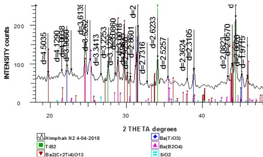
Fig. 8. The XRD pattern of the combustion products of the \text{BaCrO}_4/\text{TiB}_2 system.
