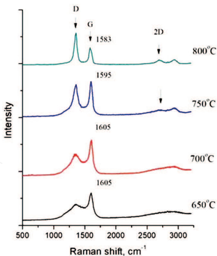
Figure 1. Raman spectra of CNT samples on a diatomite.
