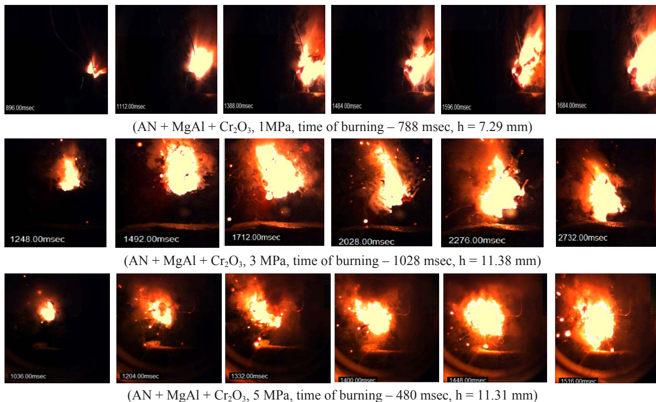
Fig. 3. Cinegrams of combustion of gas generator based on AN/MgAl/Cr 2 O 3 at 1 MPa, 3 MPa and 5 MPa.
