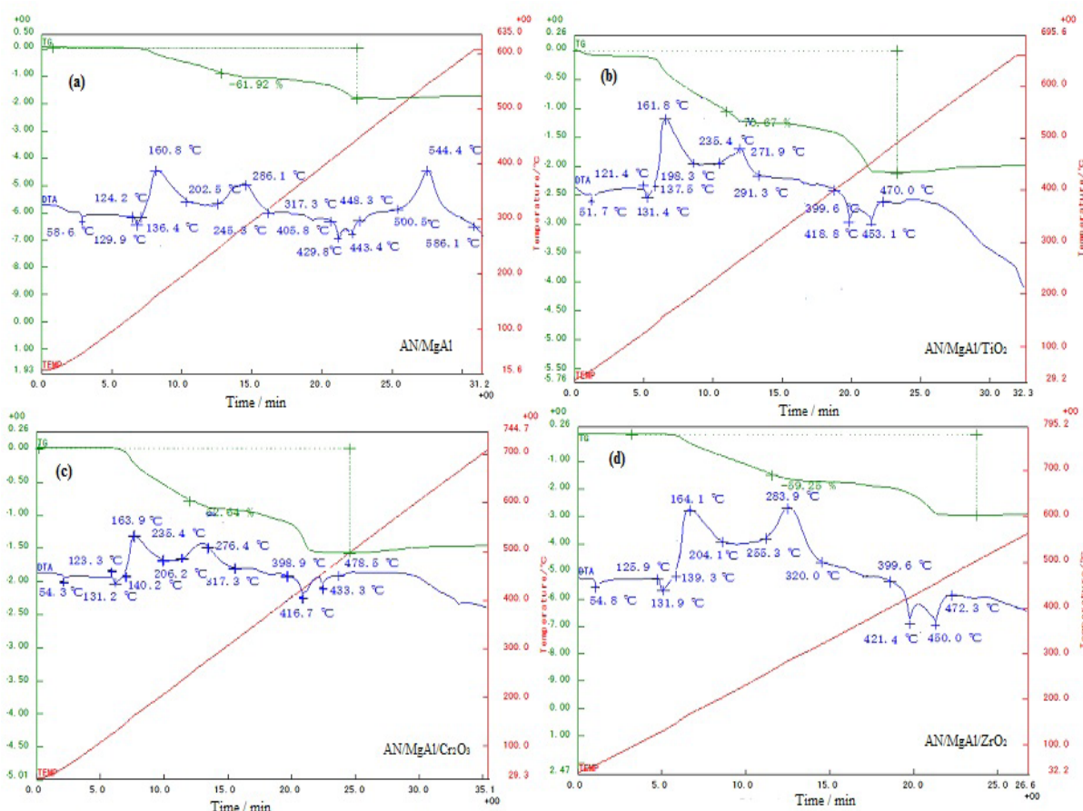
Fig. 5. The results of thermogravimetric and differential thermal analysis of the AN/MgAl and AN/MgAl/MeOx – based composite gas generators.
