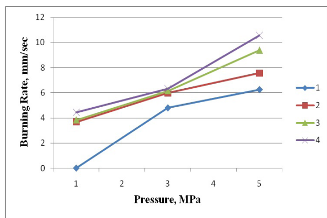
Fig. 4. Graph of the dependence of the burning rate on the pressure of the nitrogen gas: 1 – AN/MgAl; 2 – AN/MgAl/ TiO 2 ; 3 – AN/MgAl/ZrO 2 ; 4 – AN/MgAl/Cr 2 O 3 .
