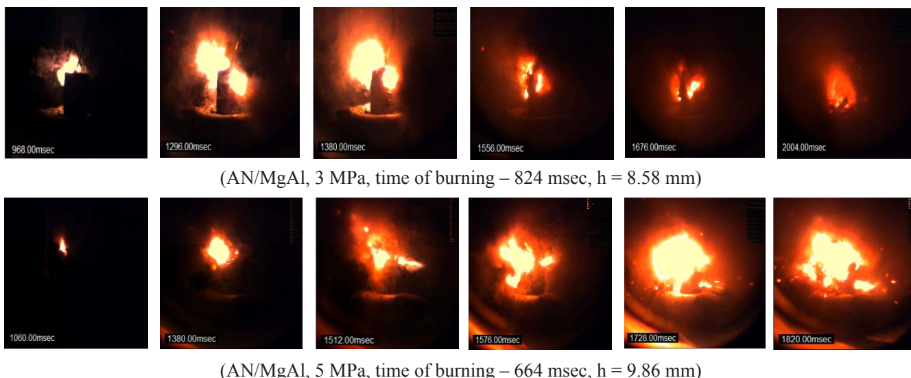
Fig. 2. Burning cinegram of the AN/MgAl-based gas generators at a pressure of 3 MPa and 5 MPa.
